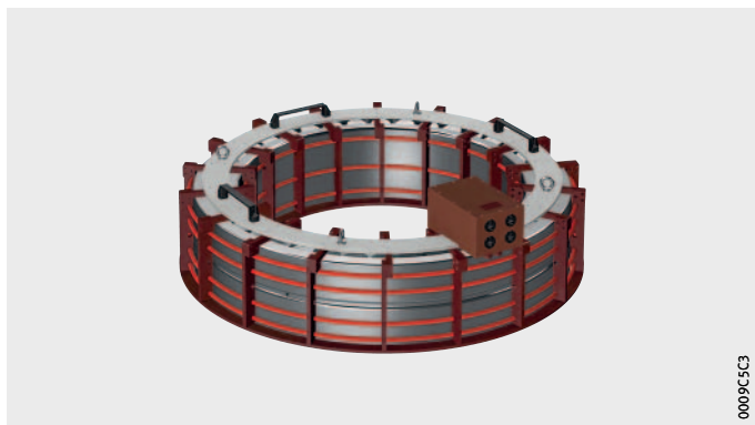
Figure 2 Twin inductor above spherical roller bearing to be heated
